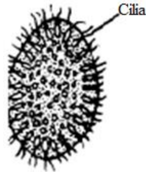
Fig 1.10 B: Synzoospores
