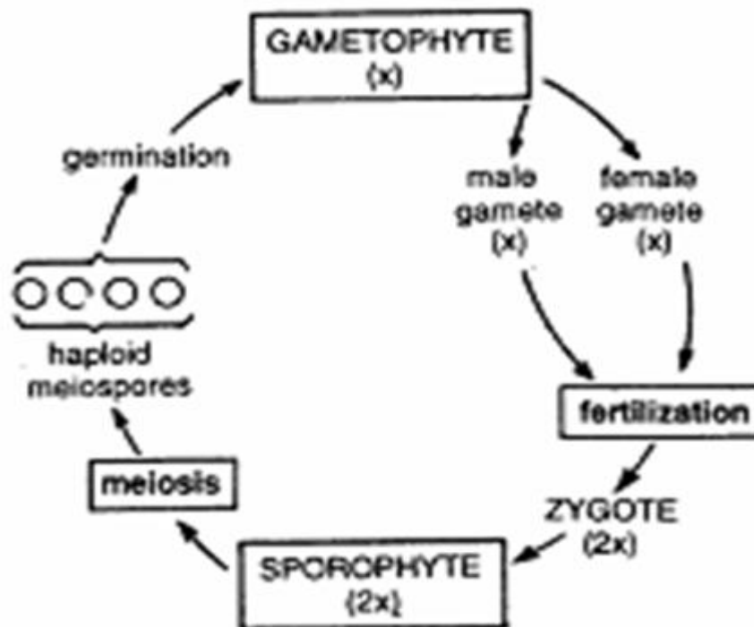
Fig.1.23: Isomorphic Type
