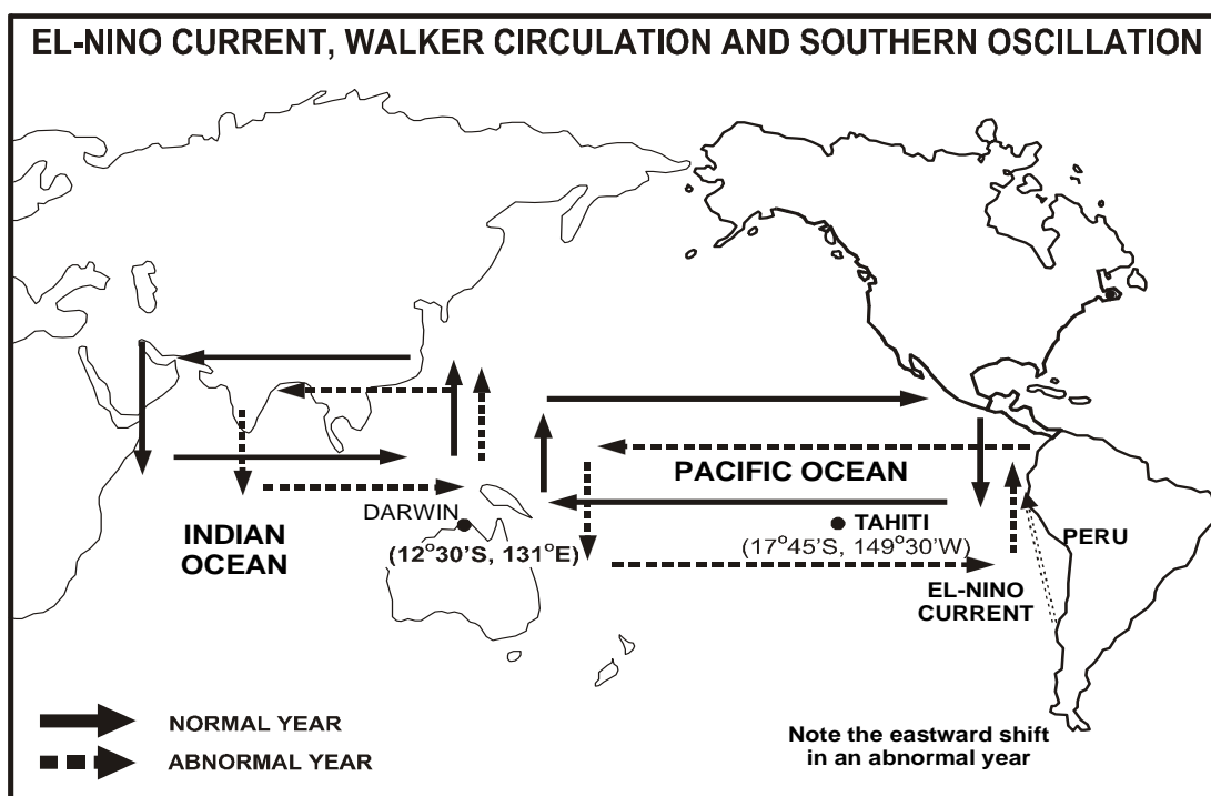
Fig.4.1 El-Nino, Walker Circulation and Southern Oscillation (By D.R. Khullar)
