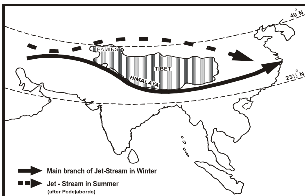
Fig. 4.5 Jet Stream (After Pedelaborde)
