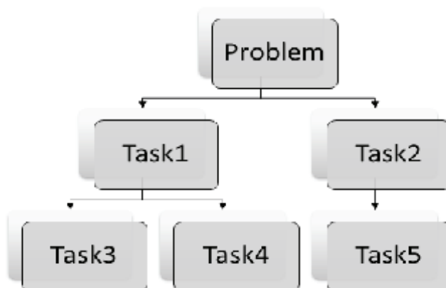
Fig. 1.6 Top-down approach
