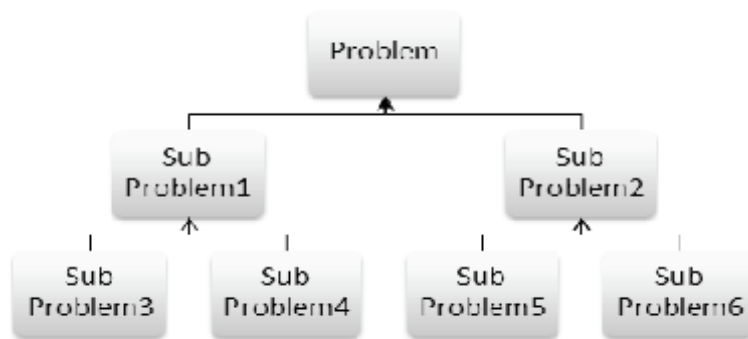
Fig. 1.7 Bottom-up approach
