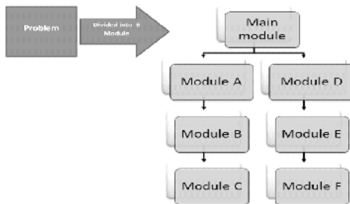
Fig. 1.8 Modular technique
